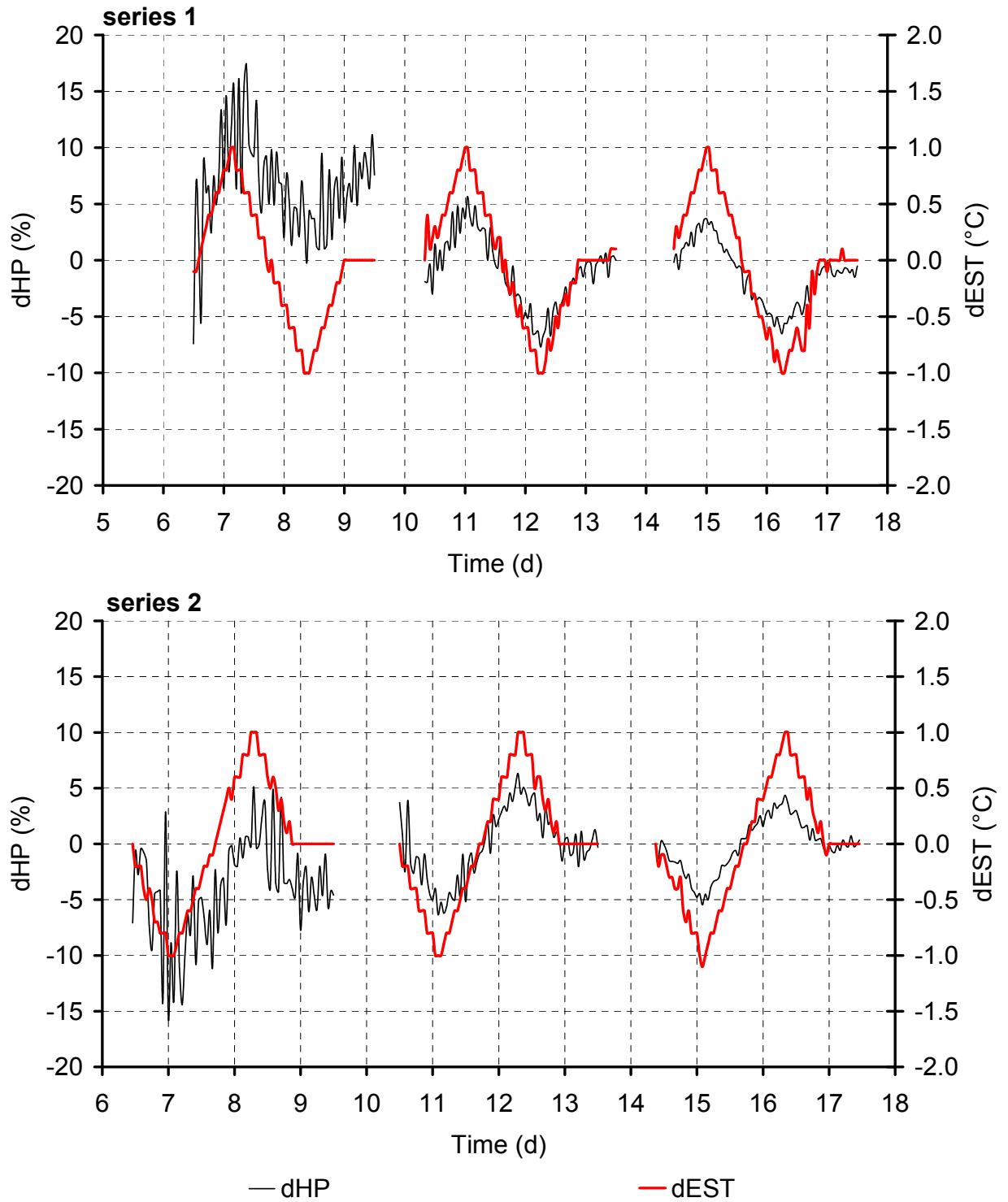
Figure 1. Relative effects of changes in eggshell temperature (dEST) away from 37.8°C on changes in heat production (dHP) in series 1 (top) and series 2 (bottom).
