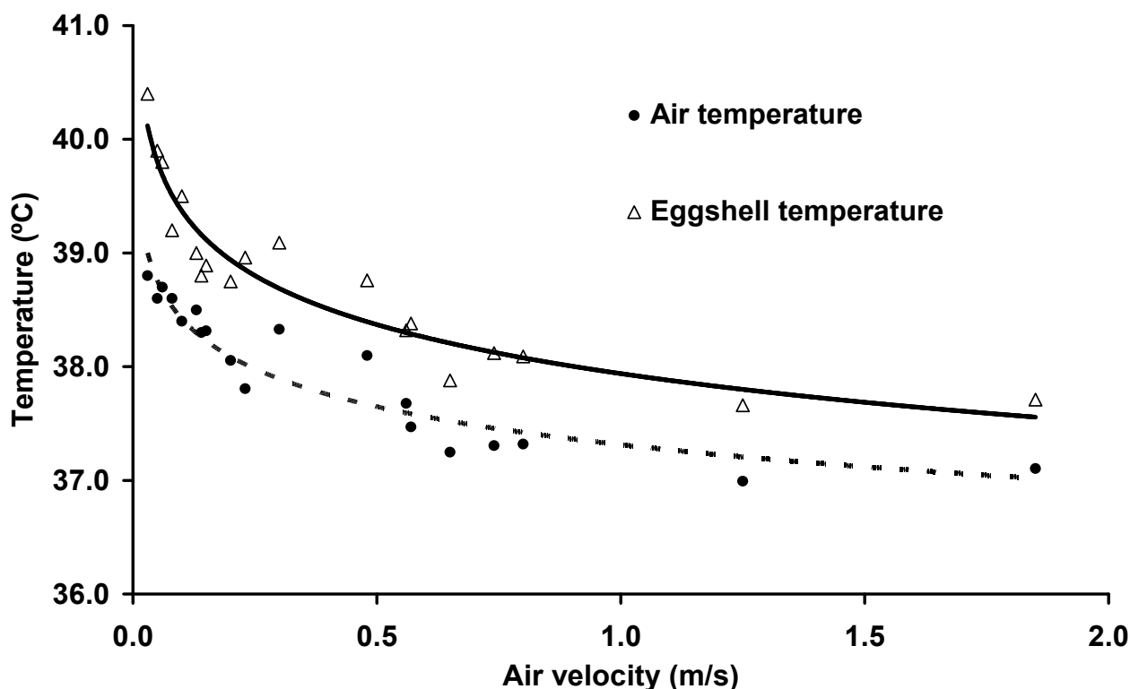
Figure 4. Effect of air velocity at a given MT of 37.2°C on air (5 cm distance from the egg) and eggshell temperature in a commercial incubator at d 18 of incubation (Lourens, 2001).
