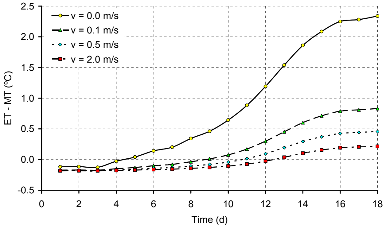
Figure 1. Development of ET during incubation, for eggs of 62g with a HP of 150 mW.egg -1 , incubated at a constant MT and at air velocities of 0.0, 0.1, 0.5 and 2.0 m.s -1 (based on calculations explained in Chapter 6).
