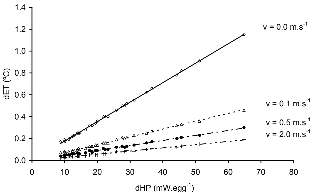
Figure 3. Calculated effects of increased heat production (dHP) on embryo temperature (dET) at d 18 of incubation as affected by air velocity.
